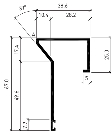
TN. 08 Modified Surround Trim
