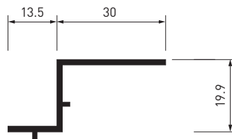
TN. 05 Aluminium Internal Corner
