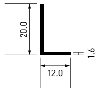
TN. 02 Aluminium Joint Angle
