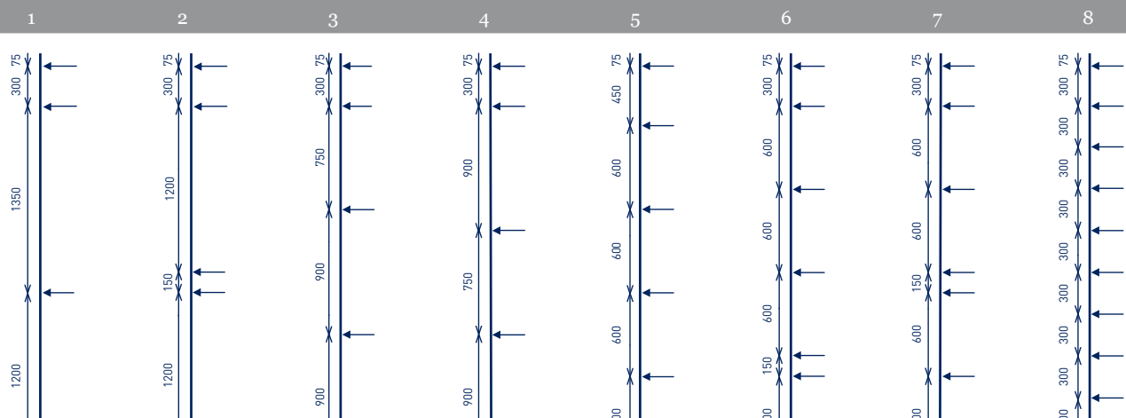
Span Configurations for Terraçade TN
