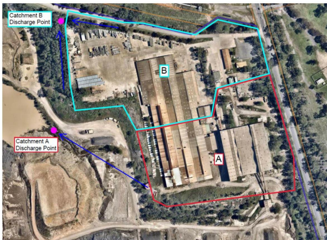
Figure 10-1 - Existing catchments for Plant 2 as shown in Figure 3 of each AT&L Civil Engineering Report
