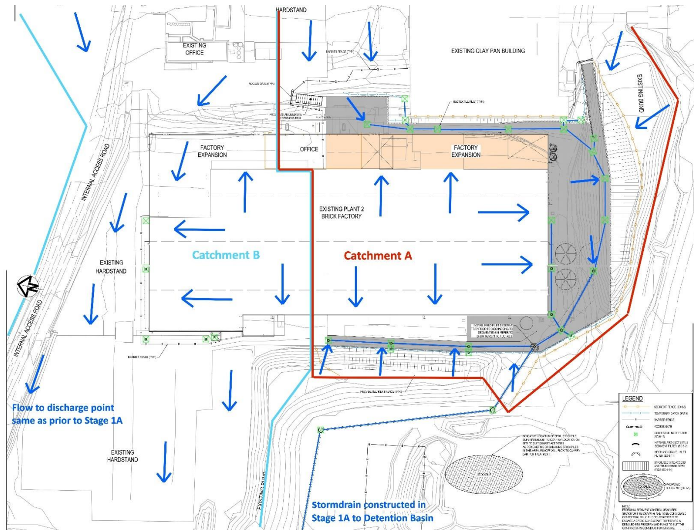
Figure 10-4 – Catchments and flow patterns for Stage 1B.
