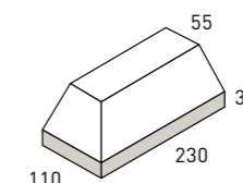
PLINTH LH EXTERNAL RETURN
