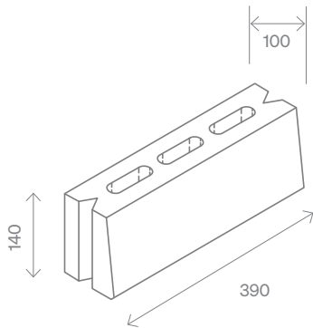
Standard Block
