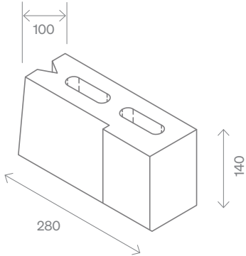
Left Hand Internal Corner
