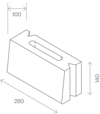
Right Hand External Corner
