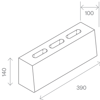
Window Block
