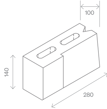
Right Hand Internal Corner
