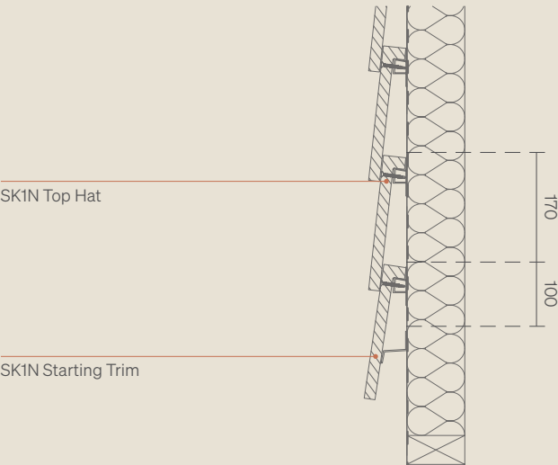
L Profile with SK1N Top Hats
