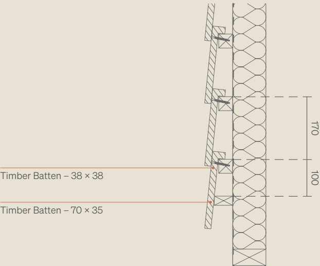
L Profile with Timber Battens
