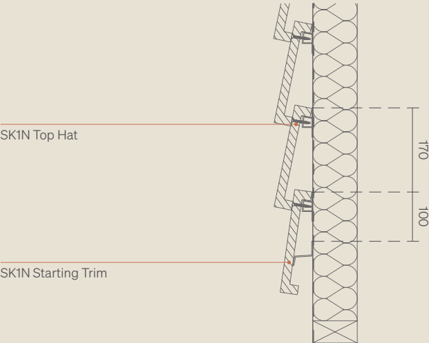
L Profile with SK1N Top Hats
