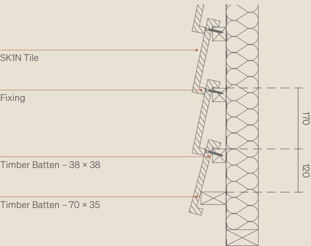
L Profile with Timber Battens
