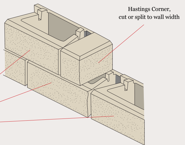
Detail for Stepping Down Blocks
