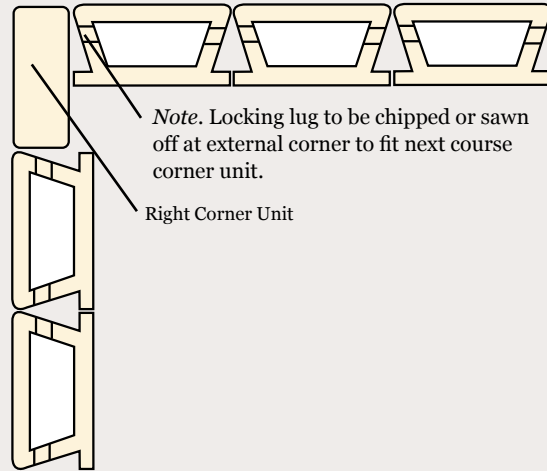
Even Courses
