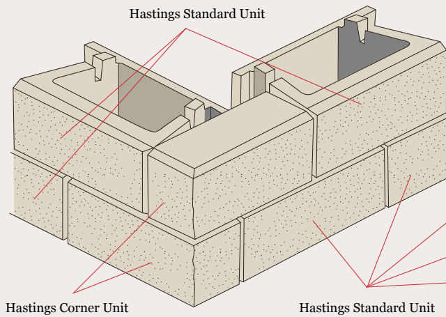
Standard 90° Corner Layout
