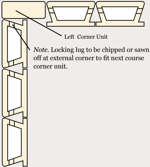
Odd Courses
